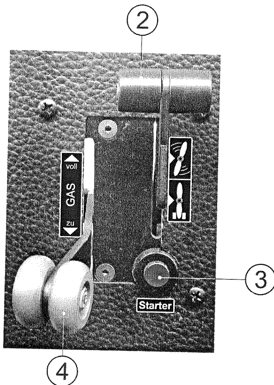
Fig. 7.7-3 Power-Plant Control Console, rear
