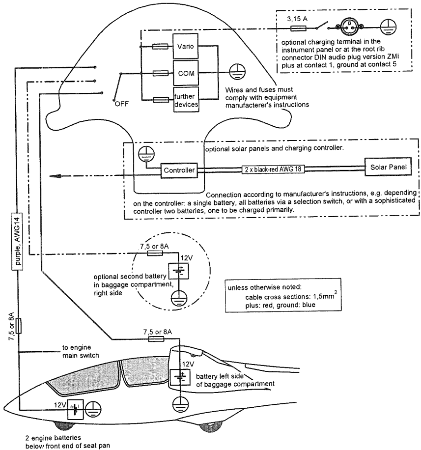
Fig. 7.9-1 On-Board Circuit
