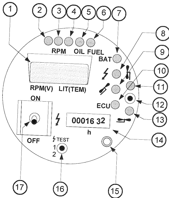
Fig. 7.7-1 ILEC Power-Plant Control Unit, Overall View
